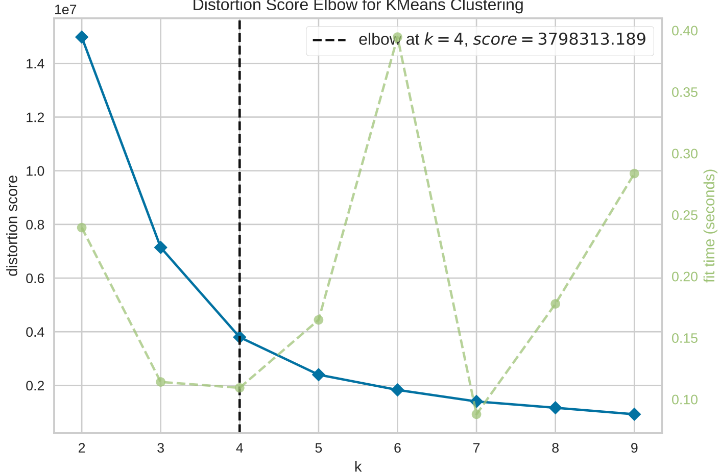
Distortion Score Elbow for KMeans Clustering
