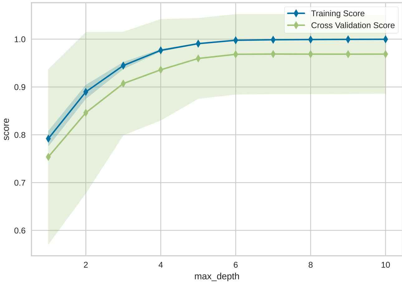
Validation Curve for DecisionTreeRegressor
