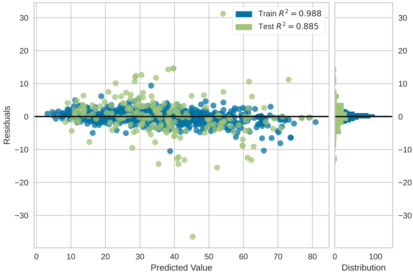
Residuals for RandomForestRegressor Model
